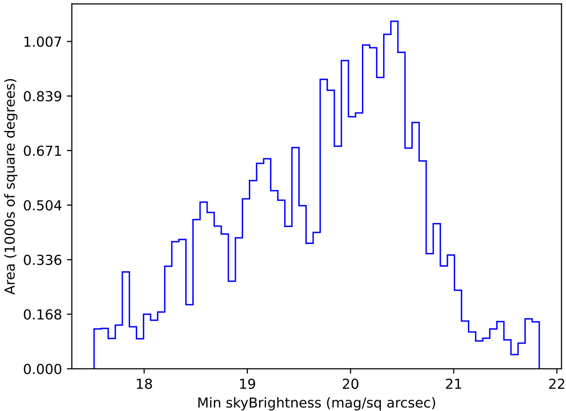
too_elab_r64_d2_gz_v3.4_10yrs All sky g band: Min skyBrightness
