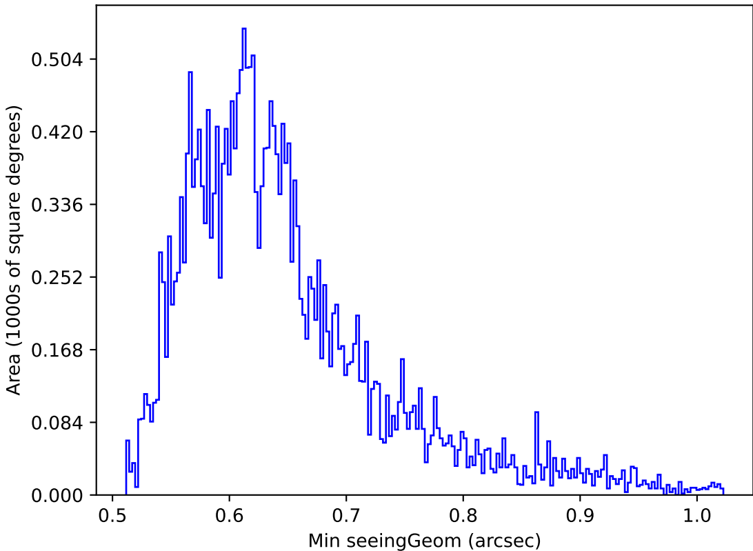
too_elab_r64_d2_gz_v3.4_10yrs Yr 1 z band: Min seeingGeom
