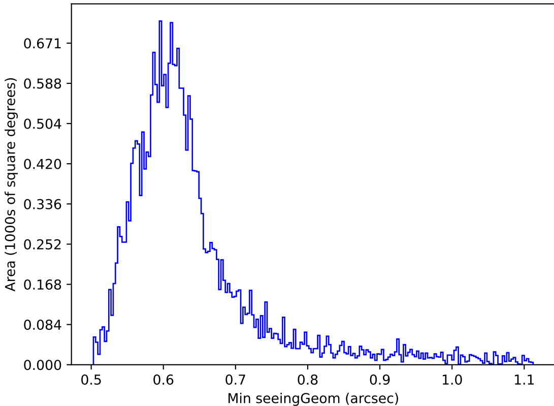
too_elab_r64_d2_gz_v3.4_10yrs Yr 1 r band: Min seeingGeom
