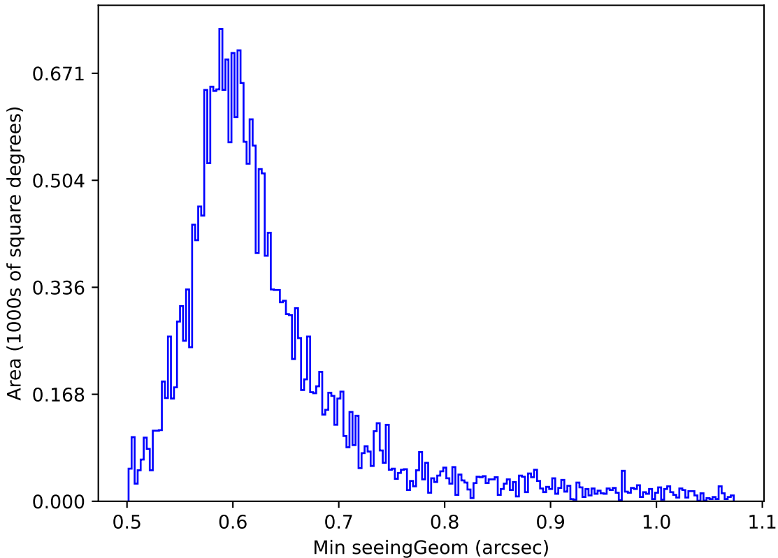
too_elab_r64_d2_gz_v3.4_10yrs Yr 1 i band: Min seeingGeom
