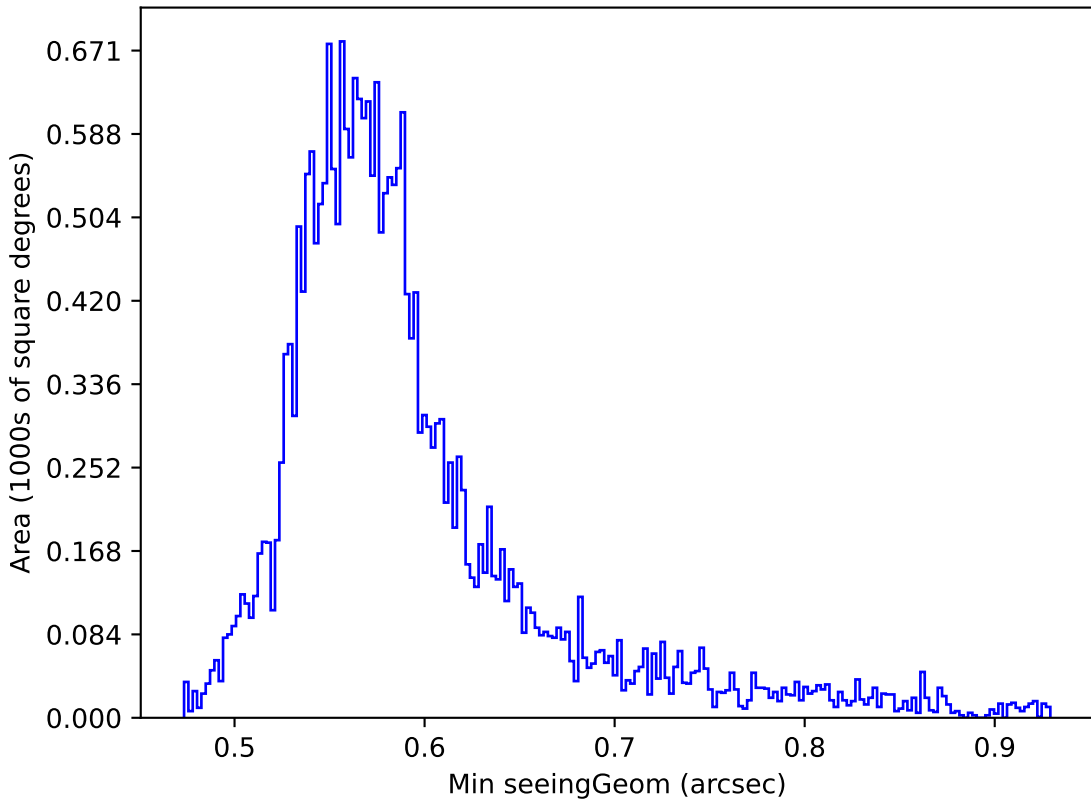
too_elab_r64_d2_gz_v3.4_10yrs Yr 1 all bands: Min seeingGeom
