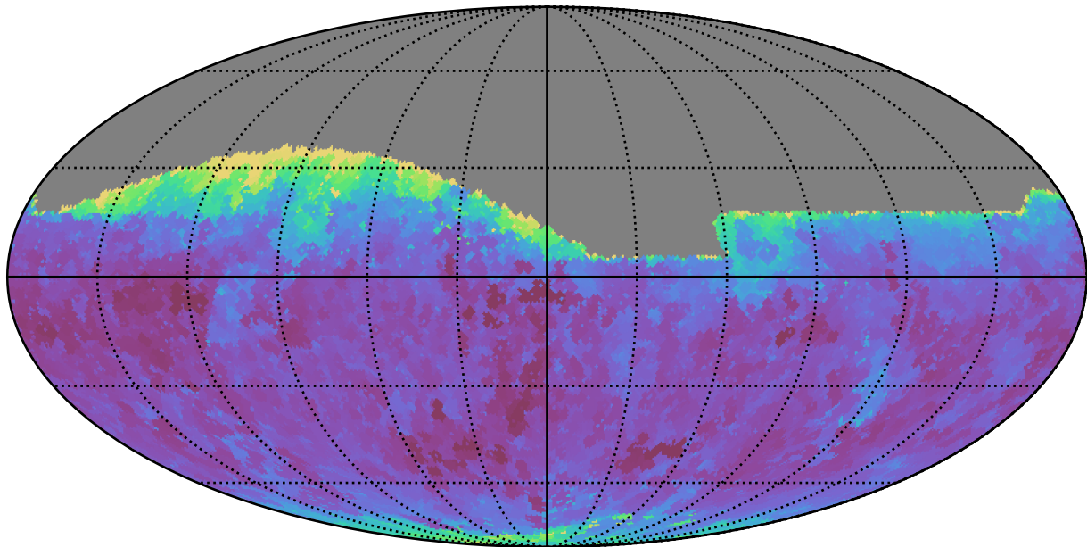
too_elab_r64_d2_gz_v3.4_10yrs Yr 1 all bands: Min seeingEff
