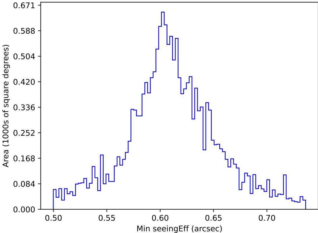
too_elab_r64_d2_gz_v3.4_10yrs WFD z band: Min seeingEff
