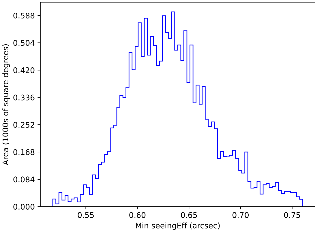
too_elab_r64_d2_gz_v3.4_10yrs WFD y band: Min seeingEff
