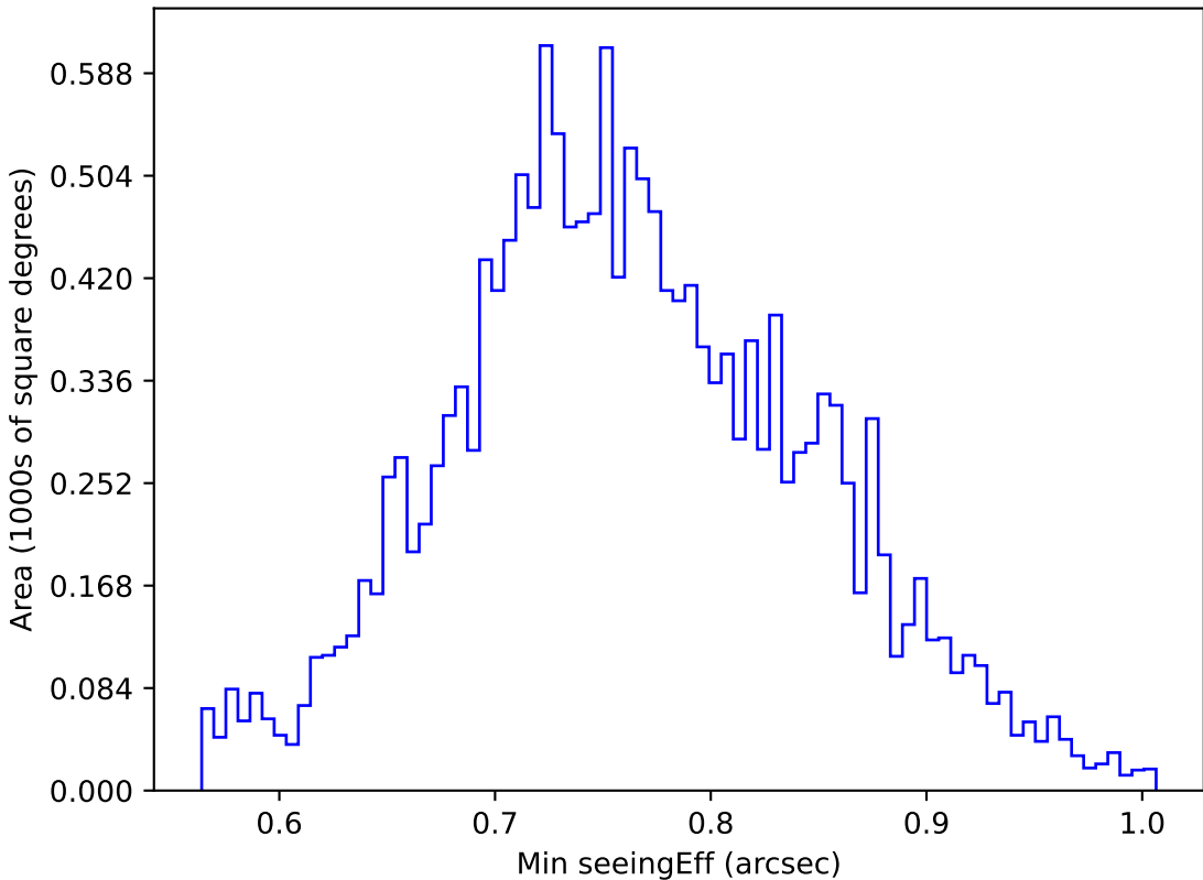
too_elab_r64_d2_gz_v3.4_10yrs WFD u band: Min seeingEff
