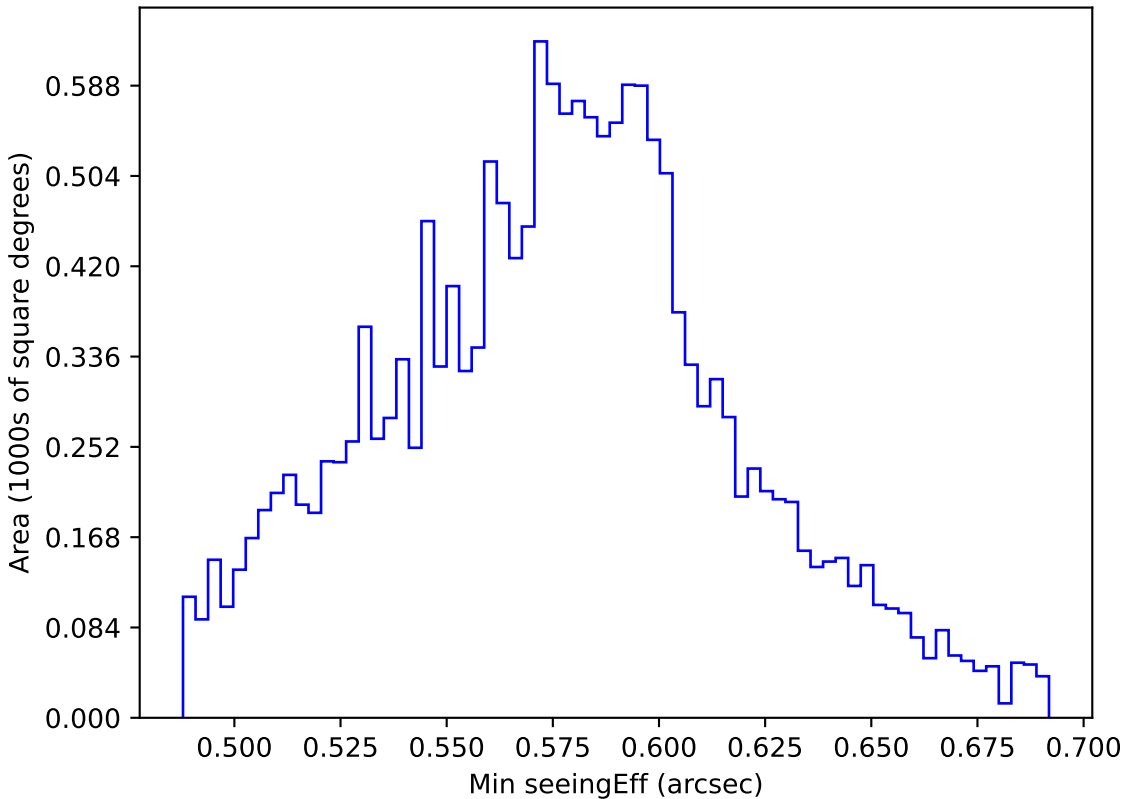
too_elab_r64_d2_gz_v3.4_10yrs WFD all bands: Min seeingEff
