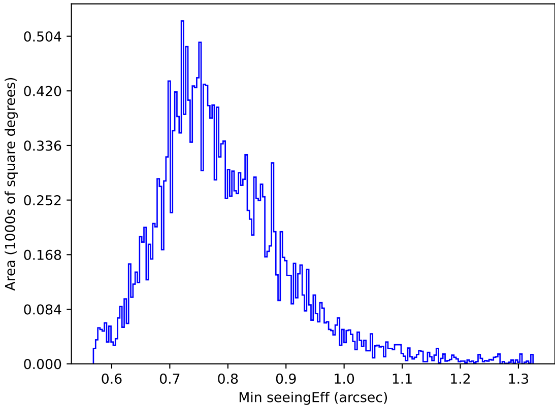
too_elab_r64_d2_gz_v3.4_10yrs All sky u band: Min seeingEff
