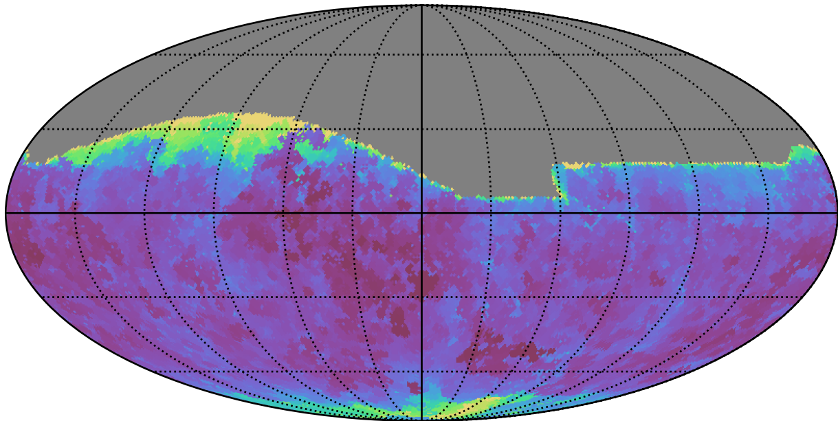
too_elab_r64_d2_gz_v3.4_10yrs All sky g band: Min seeingEff
