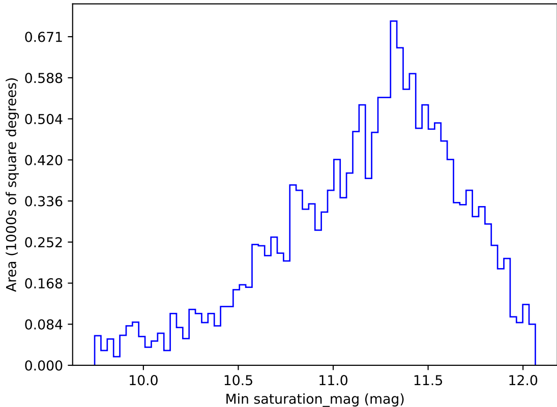
too_elab_r64_d2_gz_v3.4_10yrs WFD y band: Min saturation_mag
