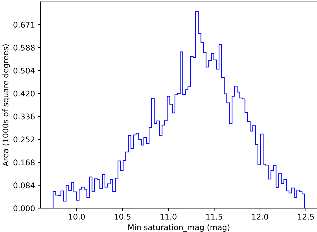
too_elab_r64_d2_gz_v3.4_10yrs All sky y band: Min saturation_mag
