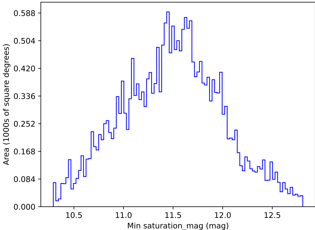
too_elab_r64_d2_gz_v3.4_10yrs All sky u band: Min saturation_mag
