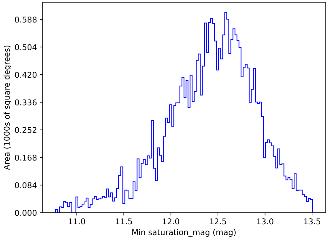
too_elab_r64_d2_gz_v3.4_10yrs All sky i band: Min saturation_mag
