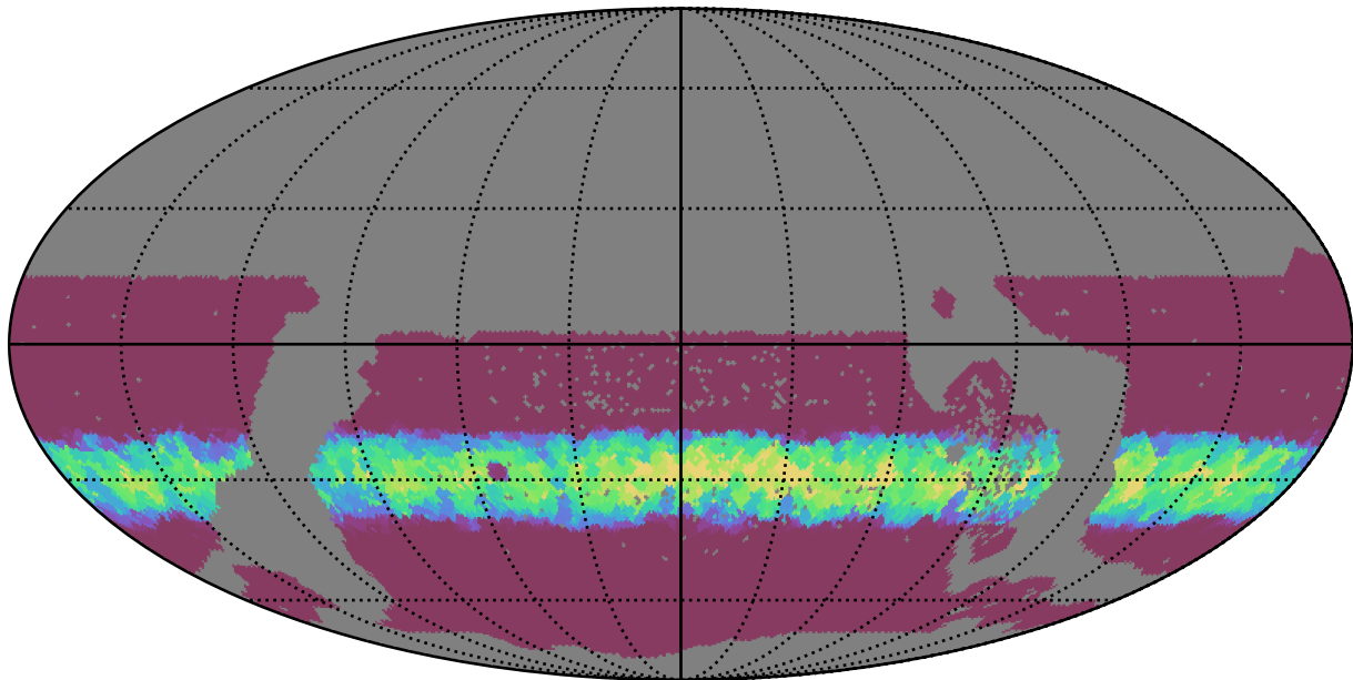
too_elab_r64_d2_gz_v3.4_10yrs WFD r band: Min normairmass
