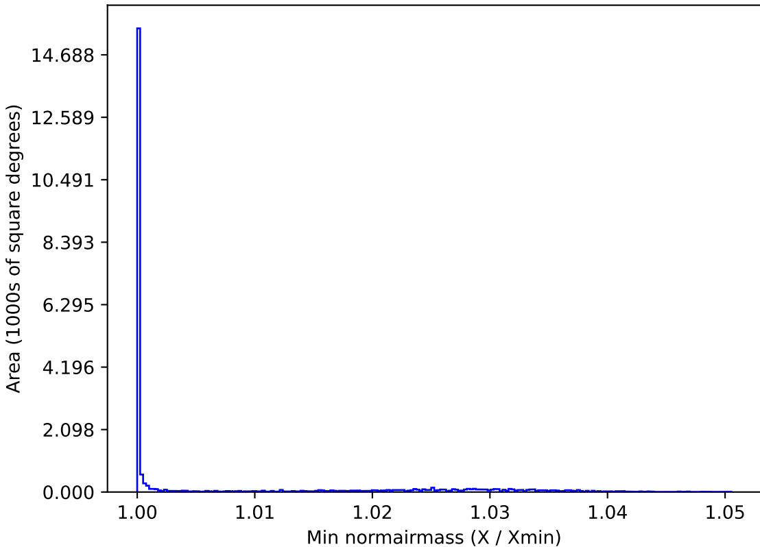
too_elab_r64_d2_gz_v3.4_10yrs All sky y band: Min normairmass
