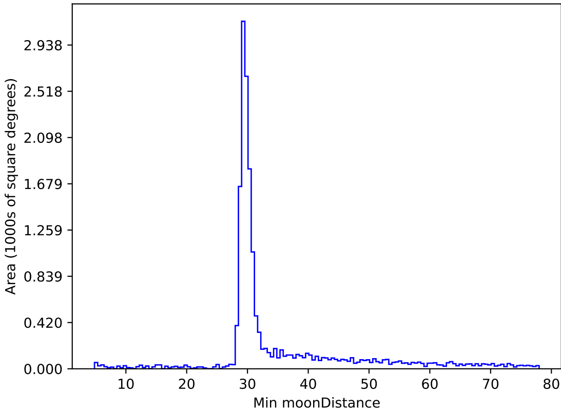
too_elab_r64_d2_gz_v3.4_10yrs WFD z band: Min moonDistance
