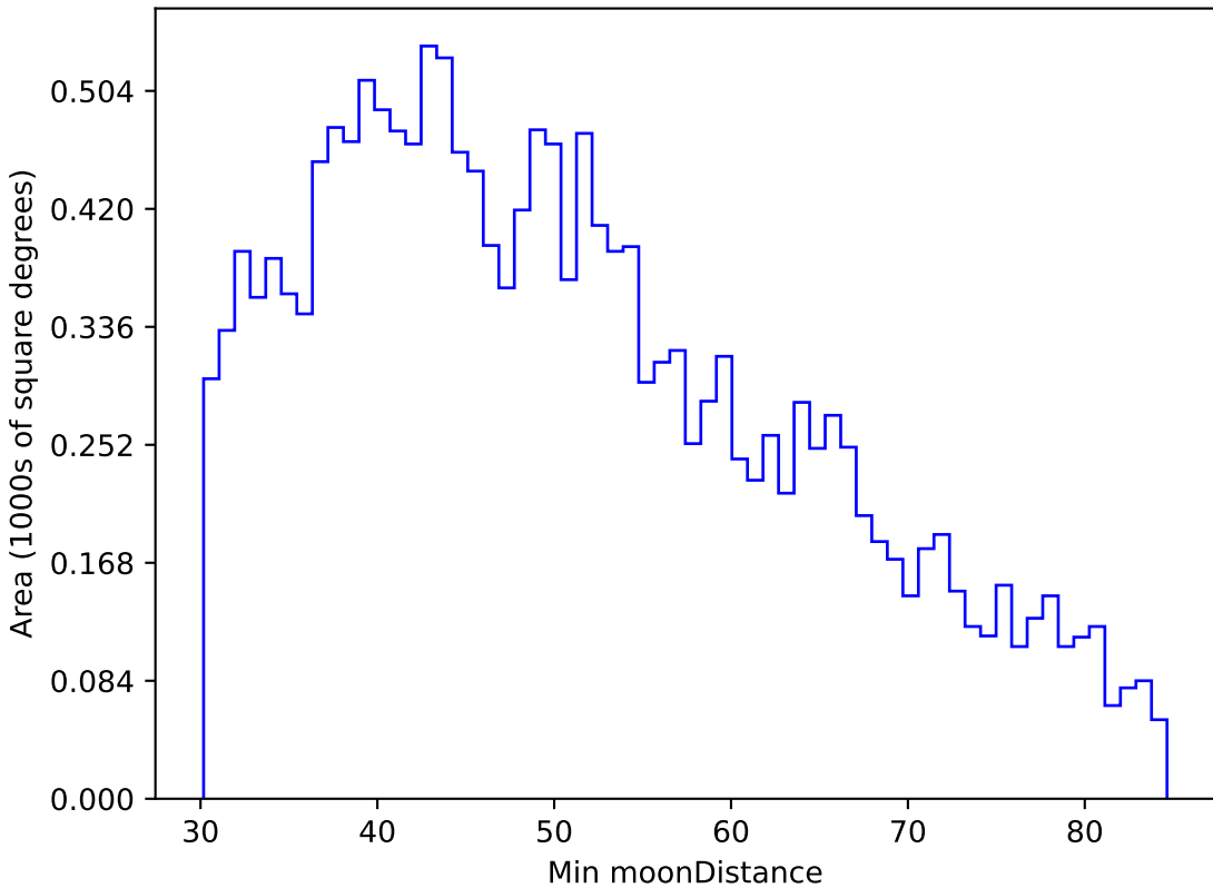
too_elab_r64_d2_gz_v3.4_10yrs WFD u band: Min moonDistance
