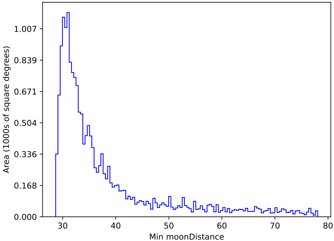
too_elab_r64_d2_gz_v3.4_10yrs WFD r band: Min moonDistance
