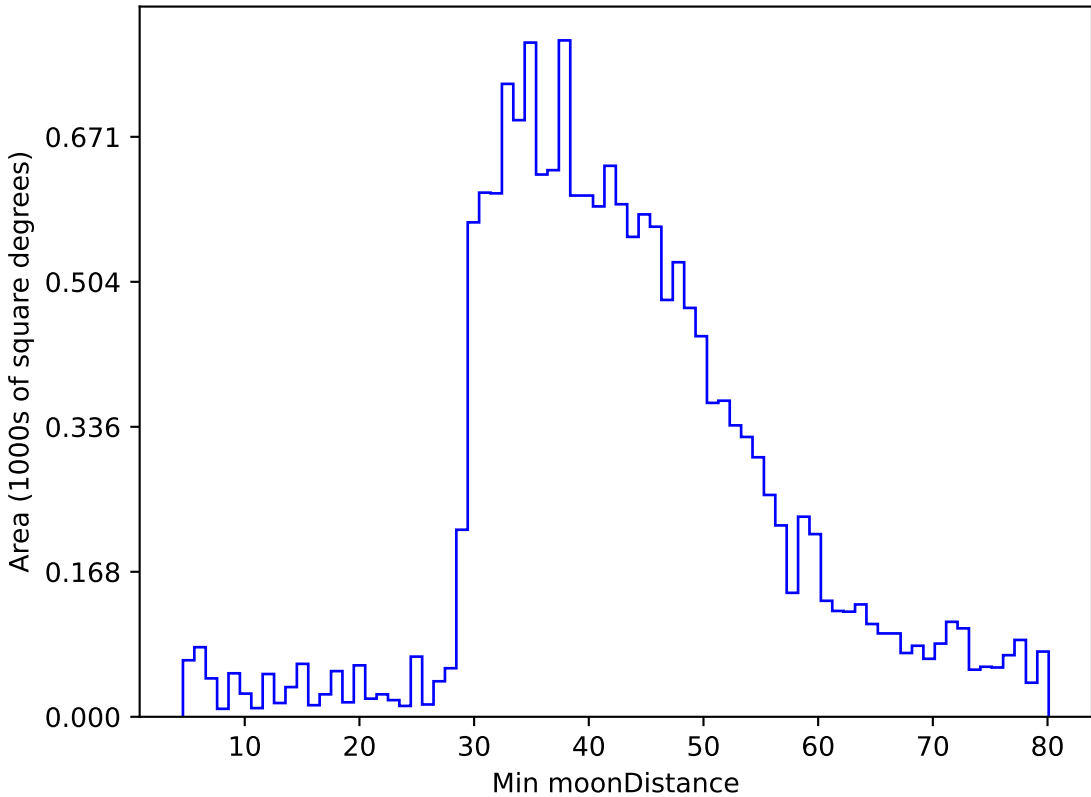
too_elab_r64_d2_gz_v3.4_10yrs WFD g band: Min moonDistance
