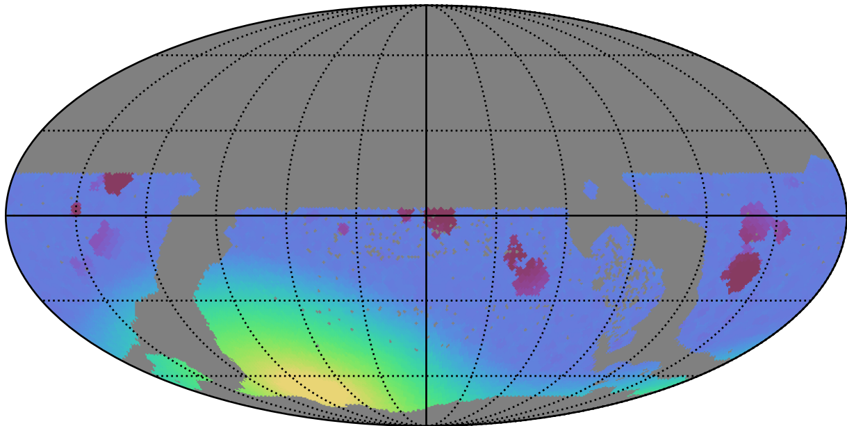
too_elab_r64_d2_gz_v3.4_10yrs WFD all bands: Min moonDistance
