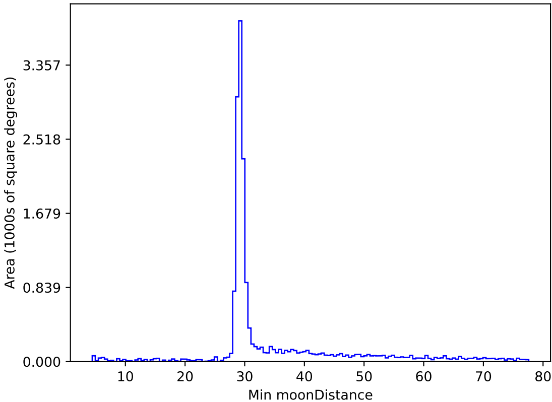
too_elab_r64_d2_gz_v3.4_10yrs WFD all bands: Min moonDistance
