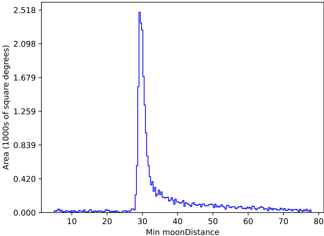
too_elab_r64_d2_gz_v3.4_10yrs All sky z band: Min moonDistance
