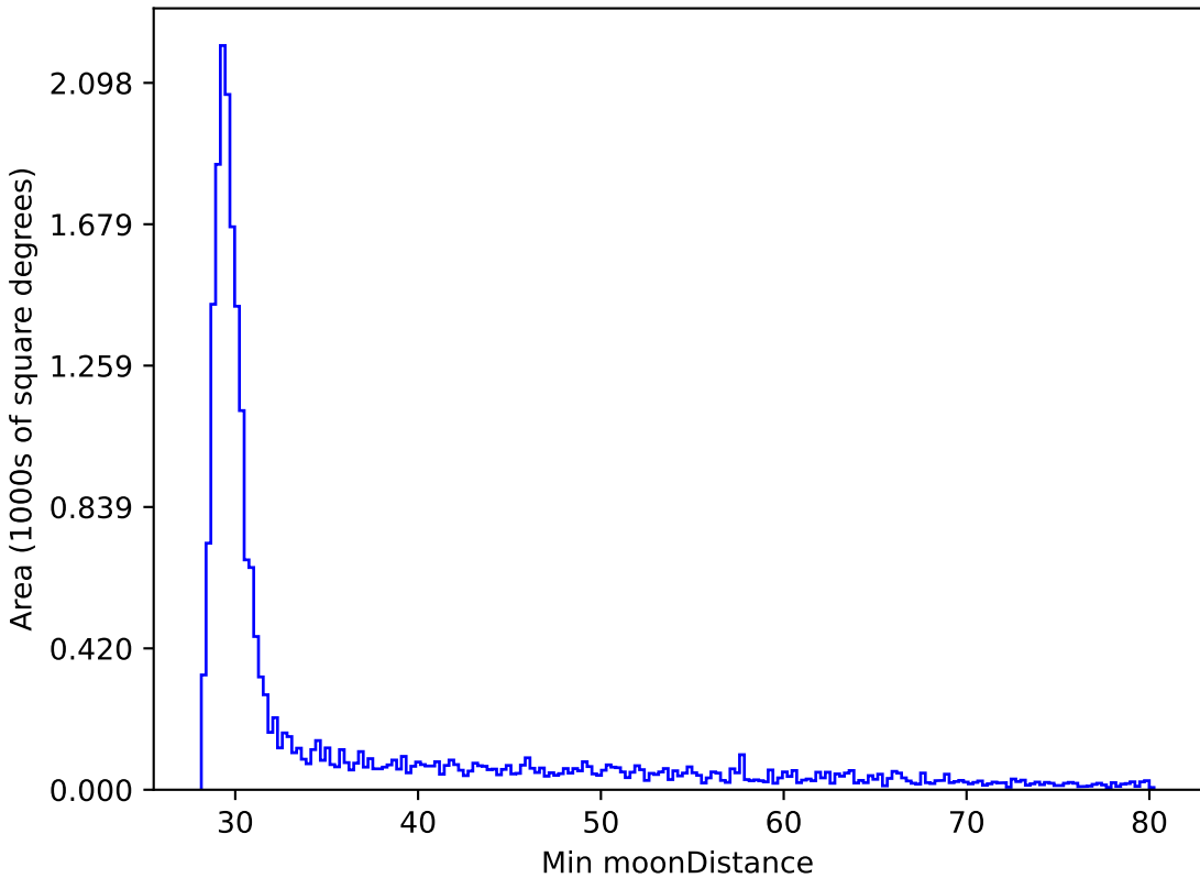
too_elab_r64_d2_gz_v3.4_10yrs All sky y band: Min moonDistance
