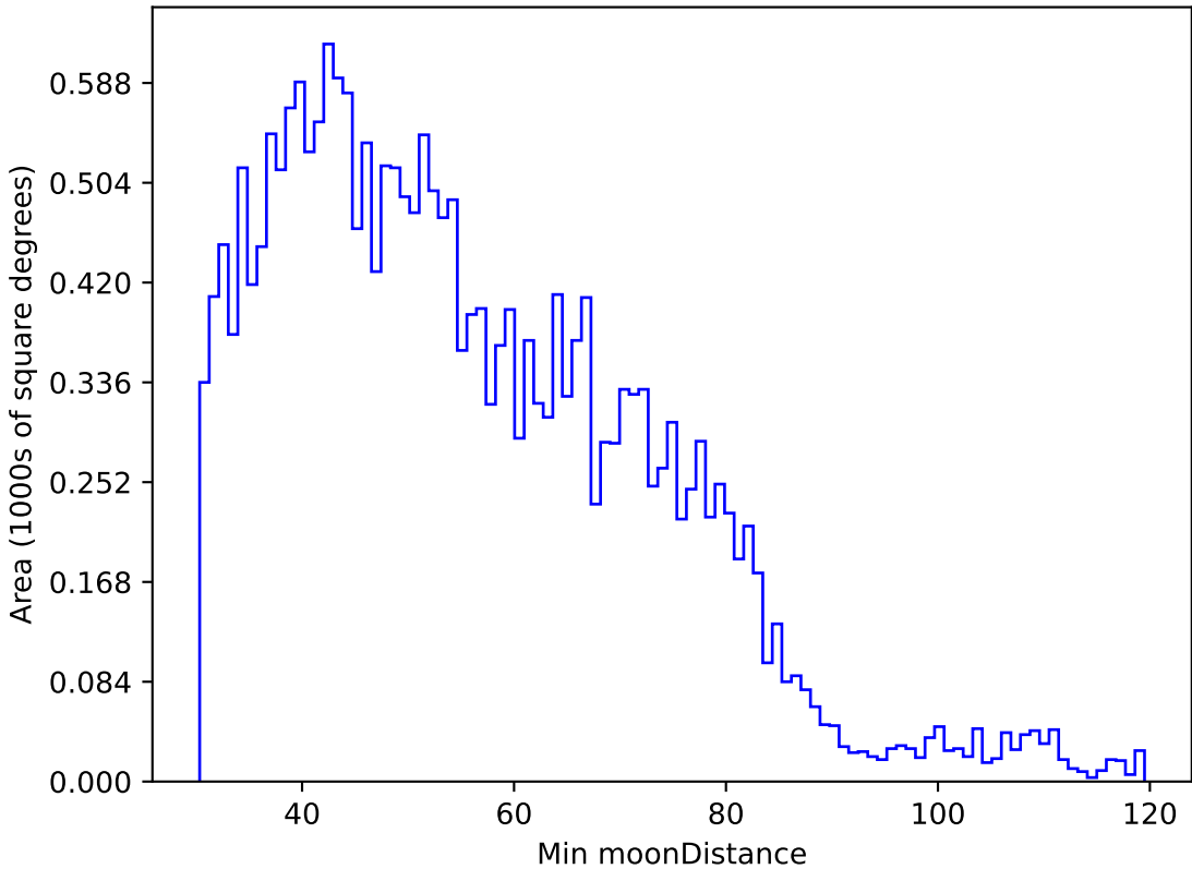
too_elab_r64_d2_gz_v3.4_10yrs All sky u band: Min moonDistance
