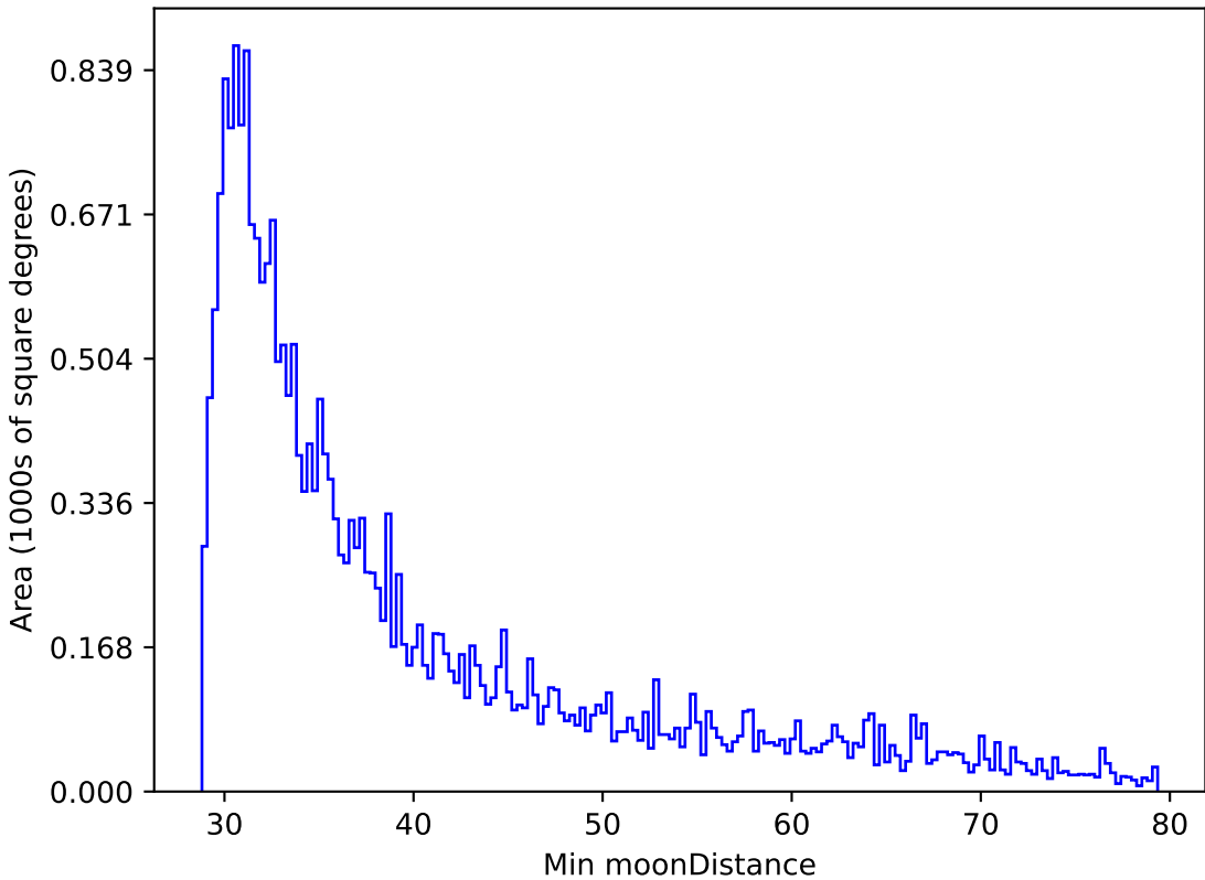
too_elab_r64_d2_gz_v3.4_10yrs All sky r band: Min moonDistance
