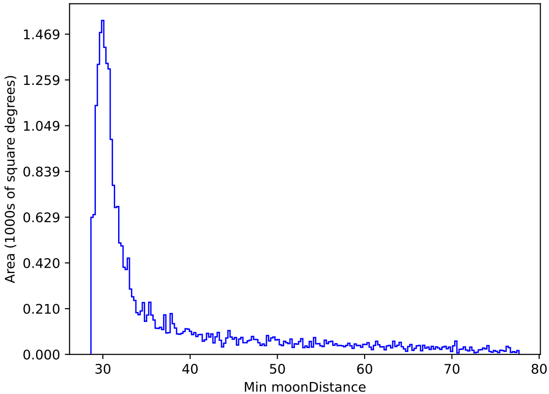
too_elab_r64_d2_gz_v3.4_10yrs All sky i band: Min moonDistance
