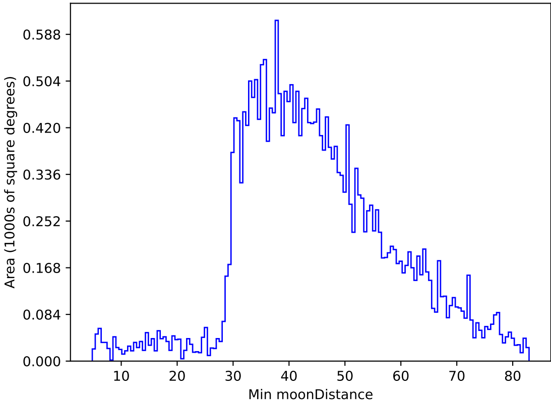
too_elab_r64_d2_gz_v3.4_10yrs All sky g band: Min moonDistance
