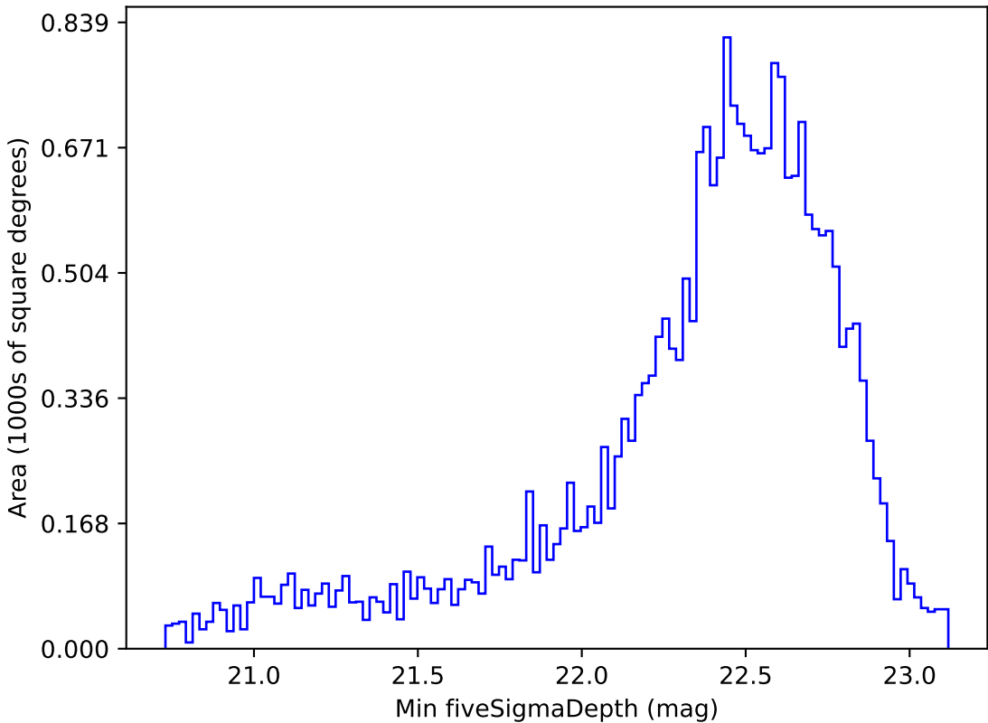
too_elab_r64_d2_gz_v3.4_10yrs Yr 1 z band: Min fiveSigmaDepth
