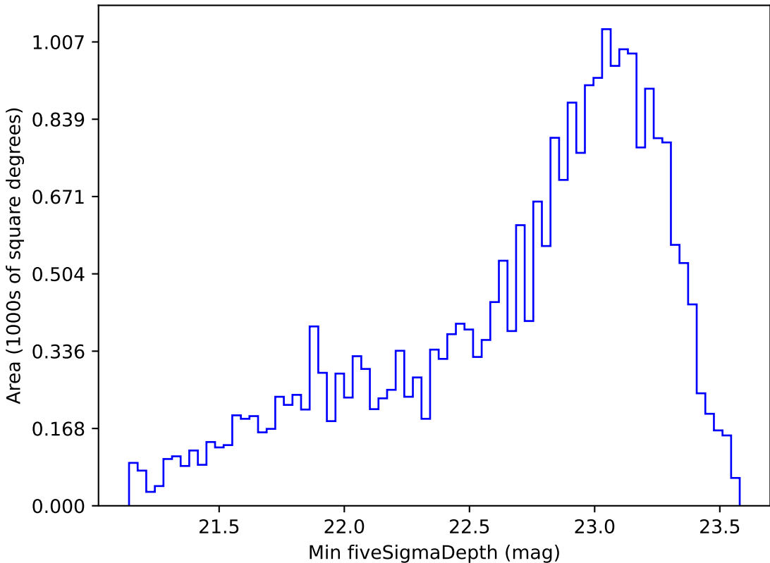
too_elab_r64_d2_gz_v3.4_10yrs Yr 1 i band: Min fiveSigmaDepth
