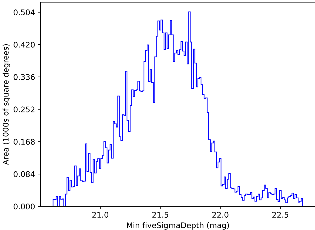
too_elab_r64_d2_gz_v3.4_10yrs Yr 1 all bands: Min fiveSigmaDepth
