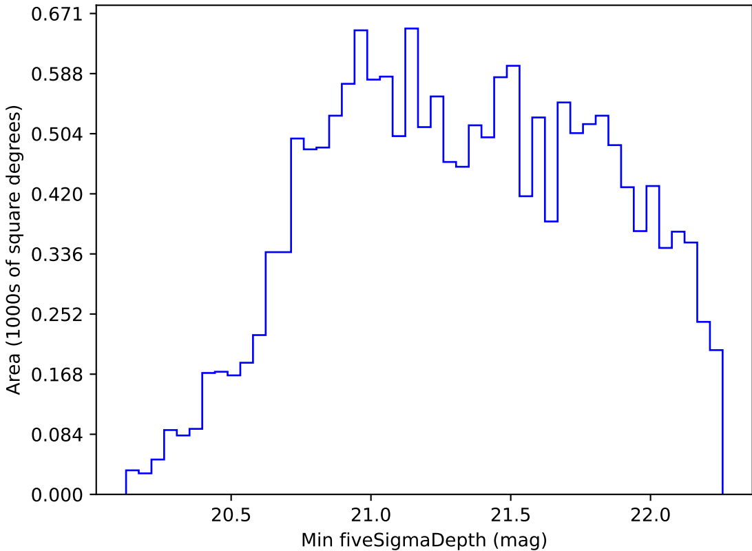
too_elab_r64_d2_gz_v3.4_10yrs WFD z band: Min fiveSigmaDepth
