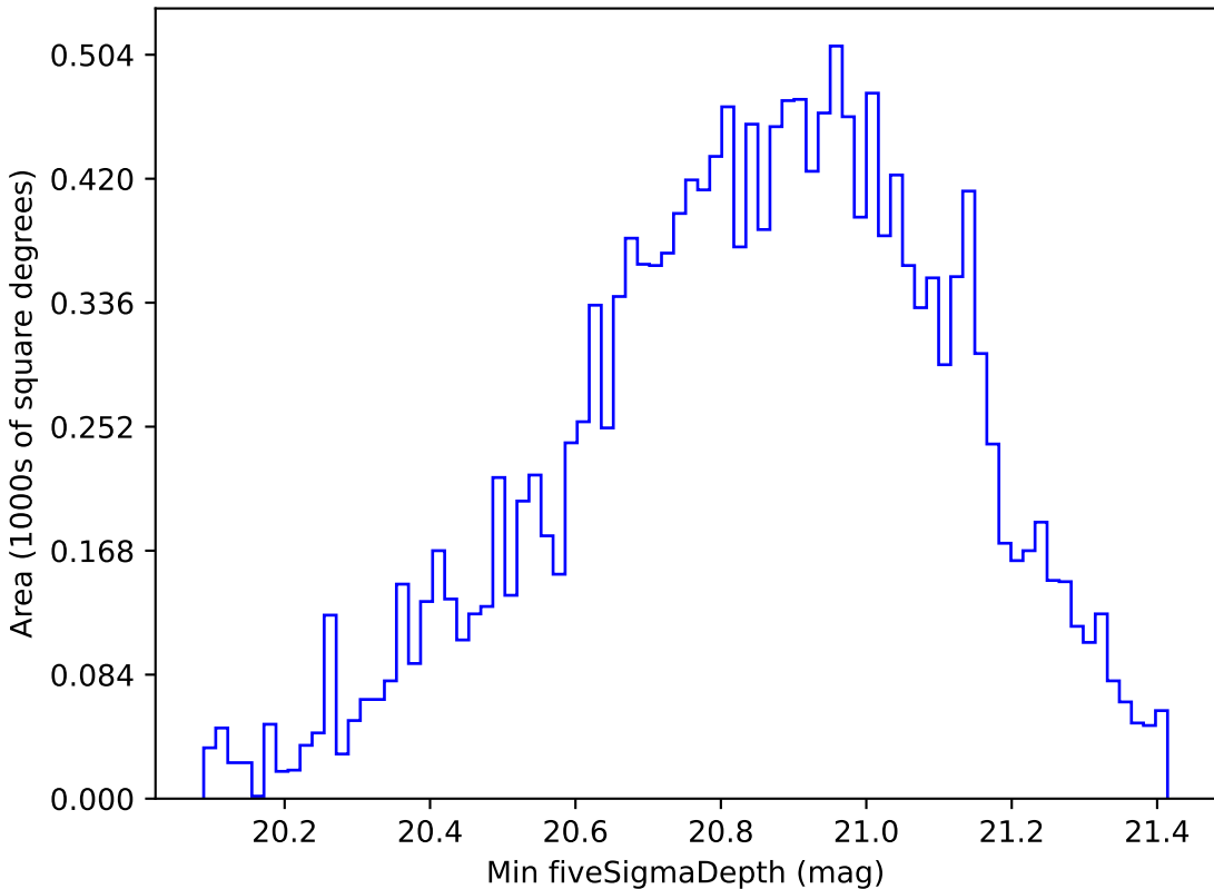
too_elab_r64_d2_gz_v3.4_10yrs WFD y band: Min fiveSigmaDepth
