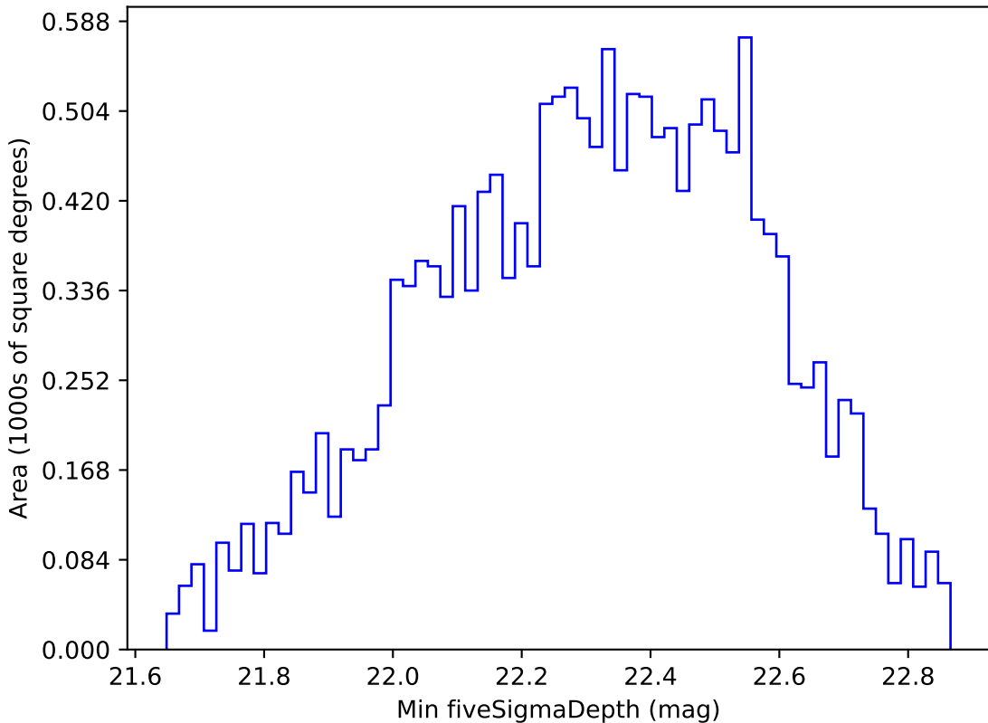
too_elab_r64_d2_gz_v3.4_10yrs WFD u band: Min fiveSigmaDepth
