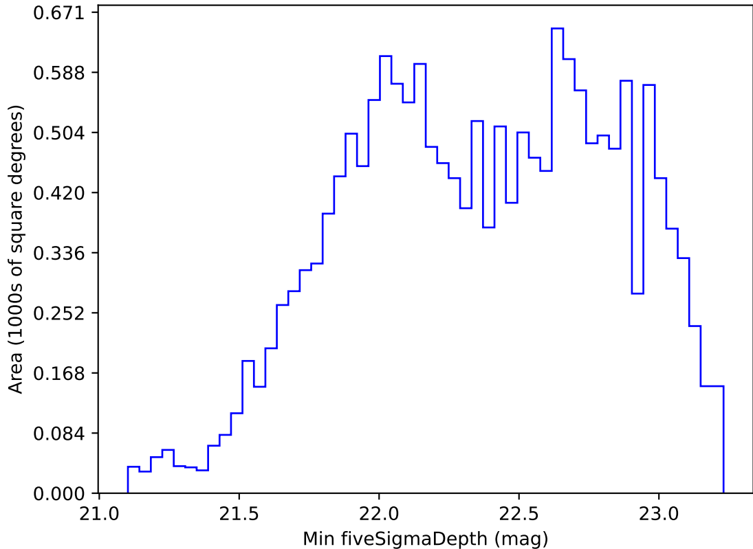
too_elab_r64_d2_gz_v3.4_10yrs WFD r band: Min fiveSigmaDepth
