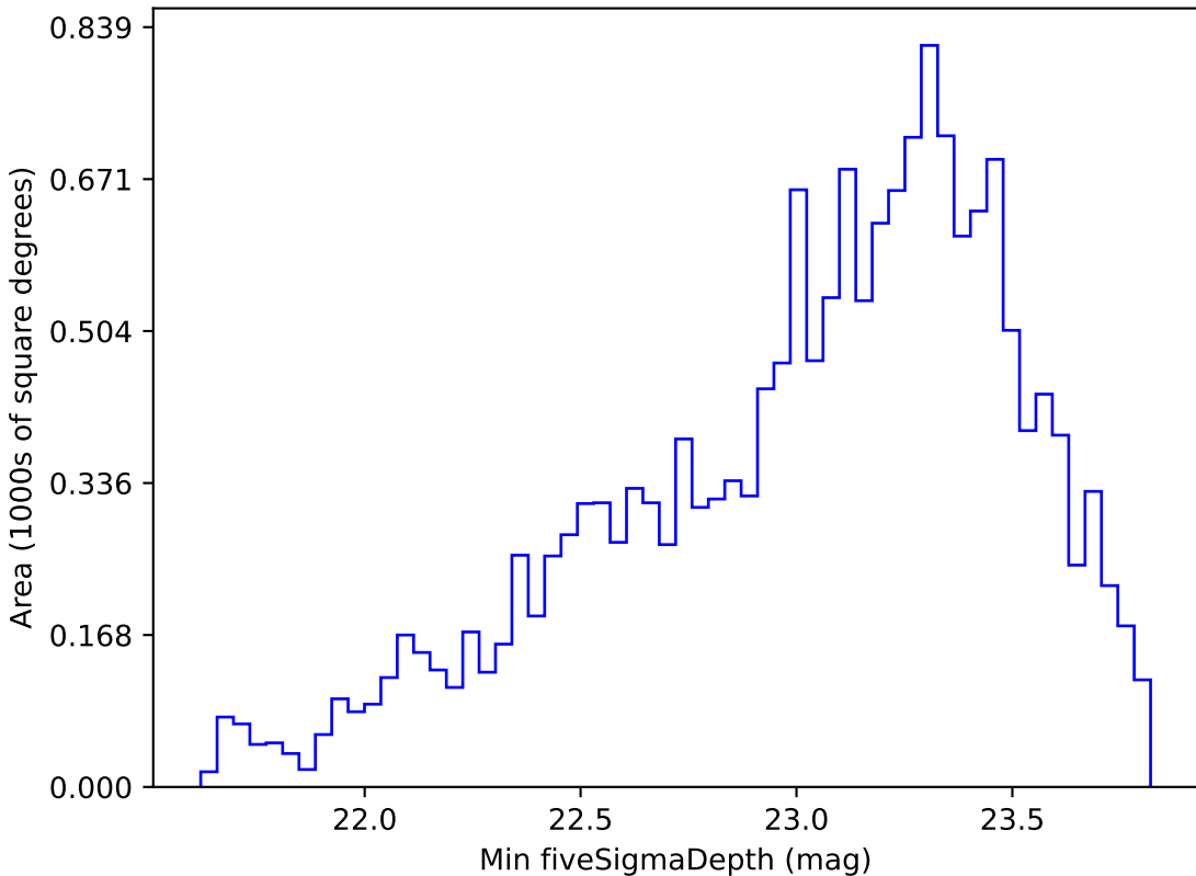
too_elab_r64_d2_gz_v3.4_10yrs WFD g band: Min fiveSigmaDepth
