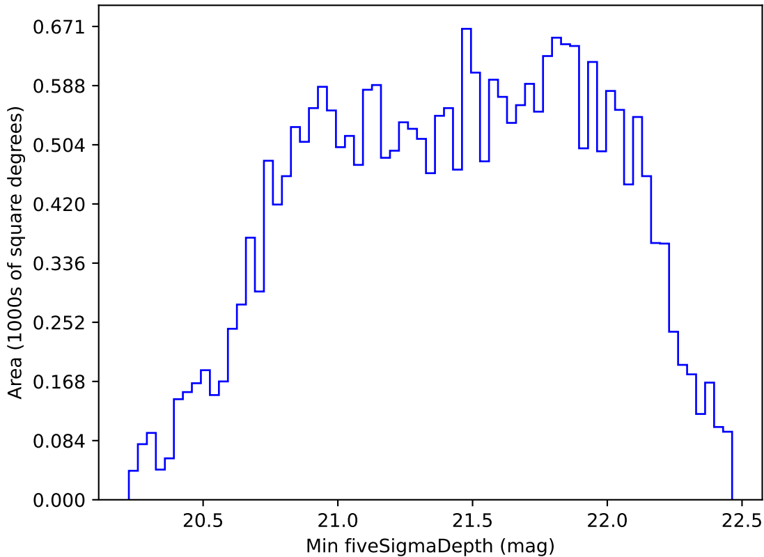
too_elab_r64_d2_gz_v3.4_10yrs All sky z band: Min fiveSigmaDepth
