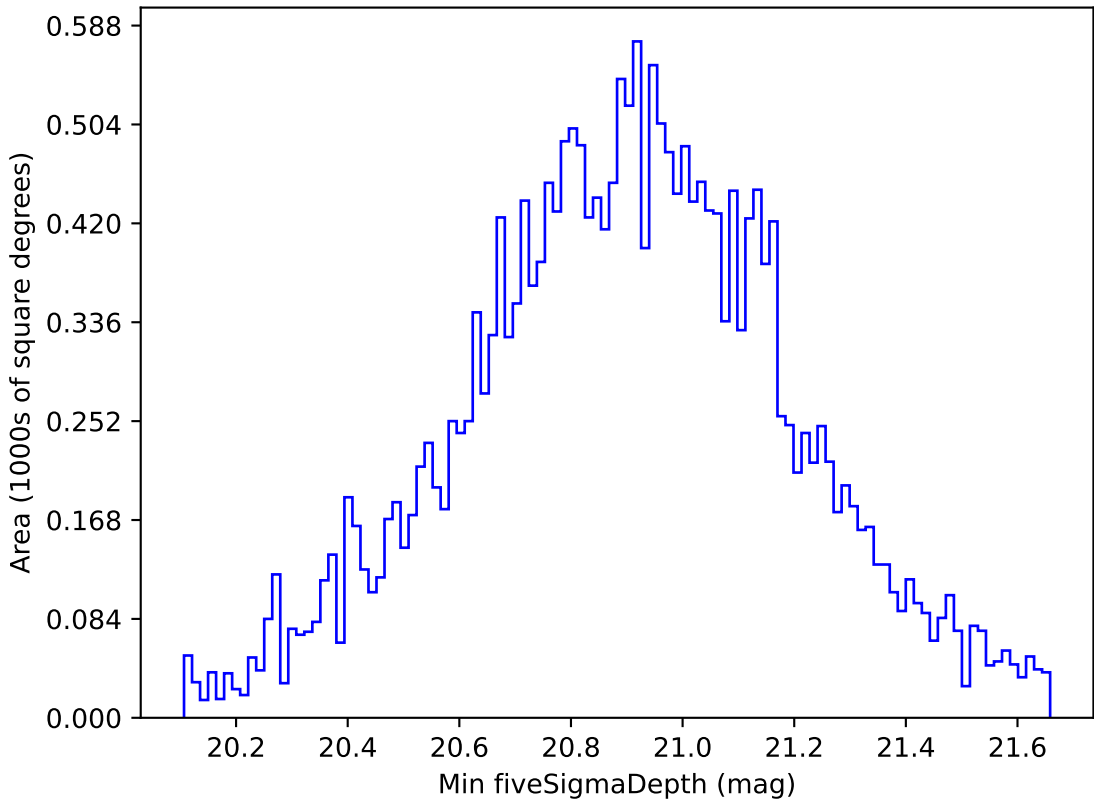
too_elab_r64_d2_gz_v3.4_10yrs All sky y band: Min fiveSigmaDepth
