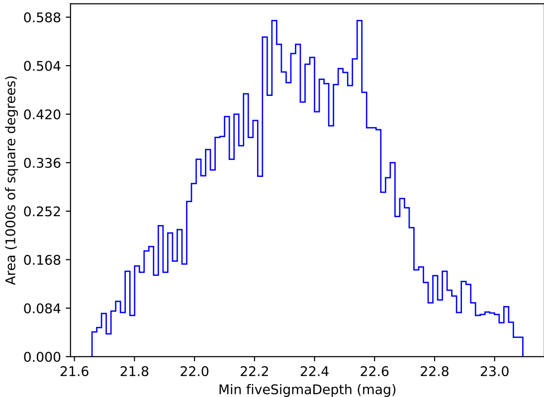
too_elab_r64_d2_gz_v3.4_10yrs All sky u band: Min fiveSigmaDepth
