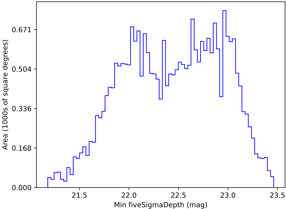
too_elab_r64_d2_gz_v3.4_10yrs All sky r band: Min fiveSigmaDepth
