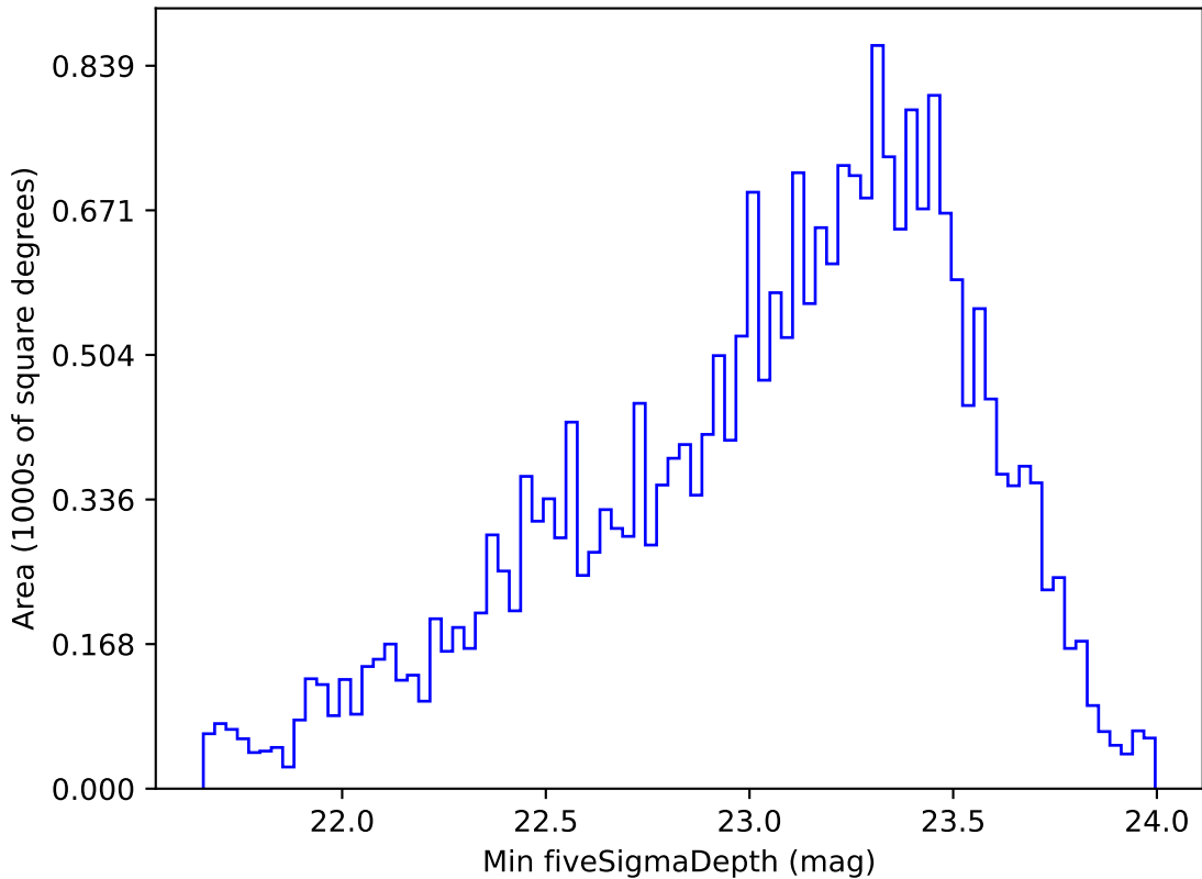
too_elab_r64_d2_gz_v3.4_10yrs All sky g band: Min fiveSigmaDepth
