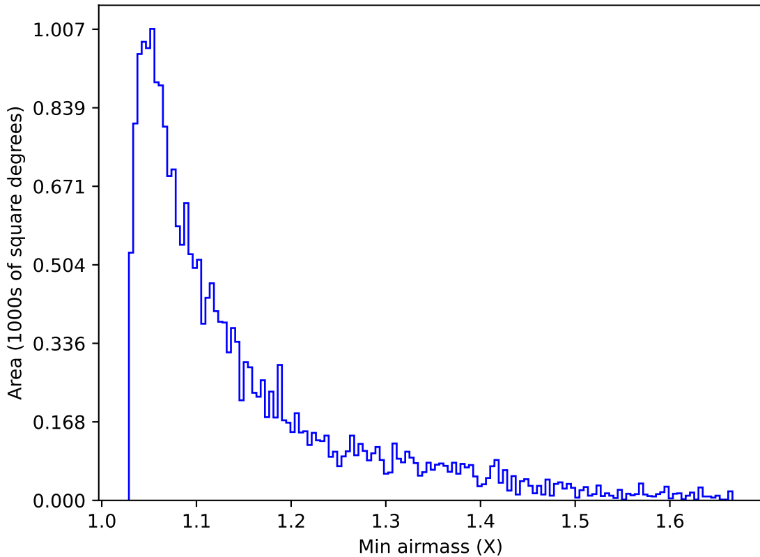
too_elab_r64_d2_gz_v3.4_10yrs Yr 1 u band: Min airmass
