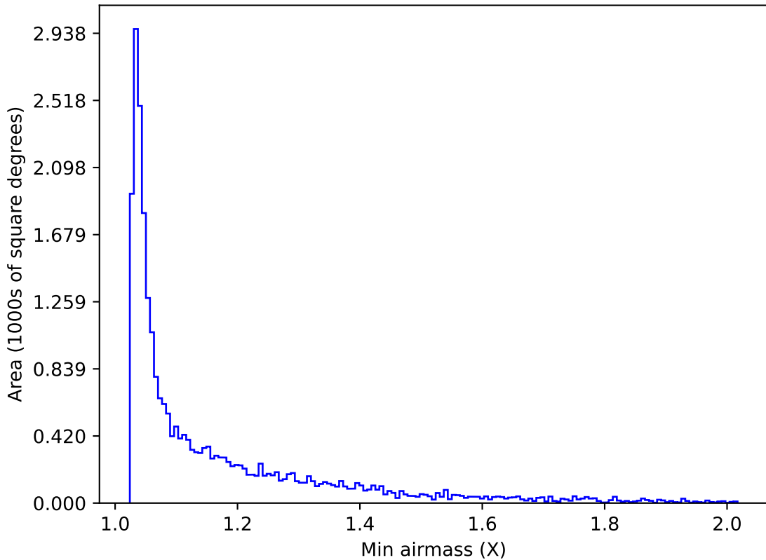
too_elab_r64_d2_gz_v3.4_10yrs Yr 1 r band: Min airmass
