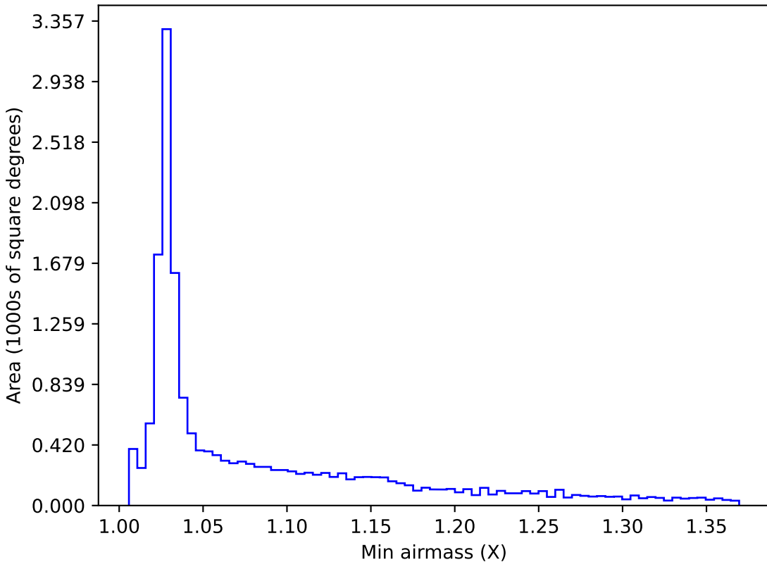
too_elab_r64_d2_gz_v3.4_10yrs WFD z band: Min airmass
