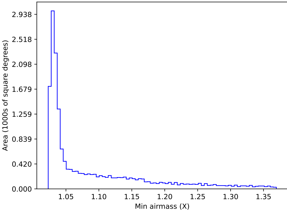
too_elab_r64_d2_gz_v3.4_10yrs WFD y band: Min airmass
