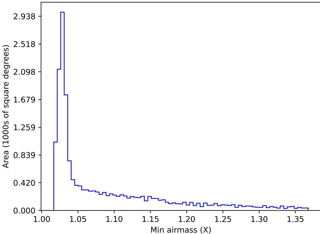
too_elab_r64_d2_gz_v3.4_10yrs WFD r band: Min airmass
