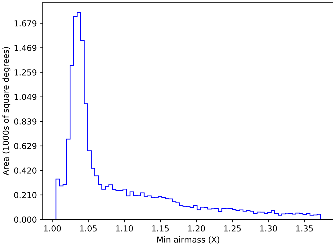
too_elab_r64_d2_gz_v3.4_10yrs WFD g band: Min airmass
