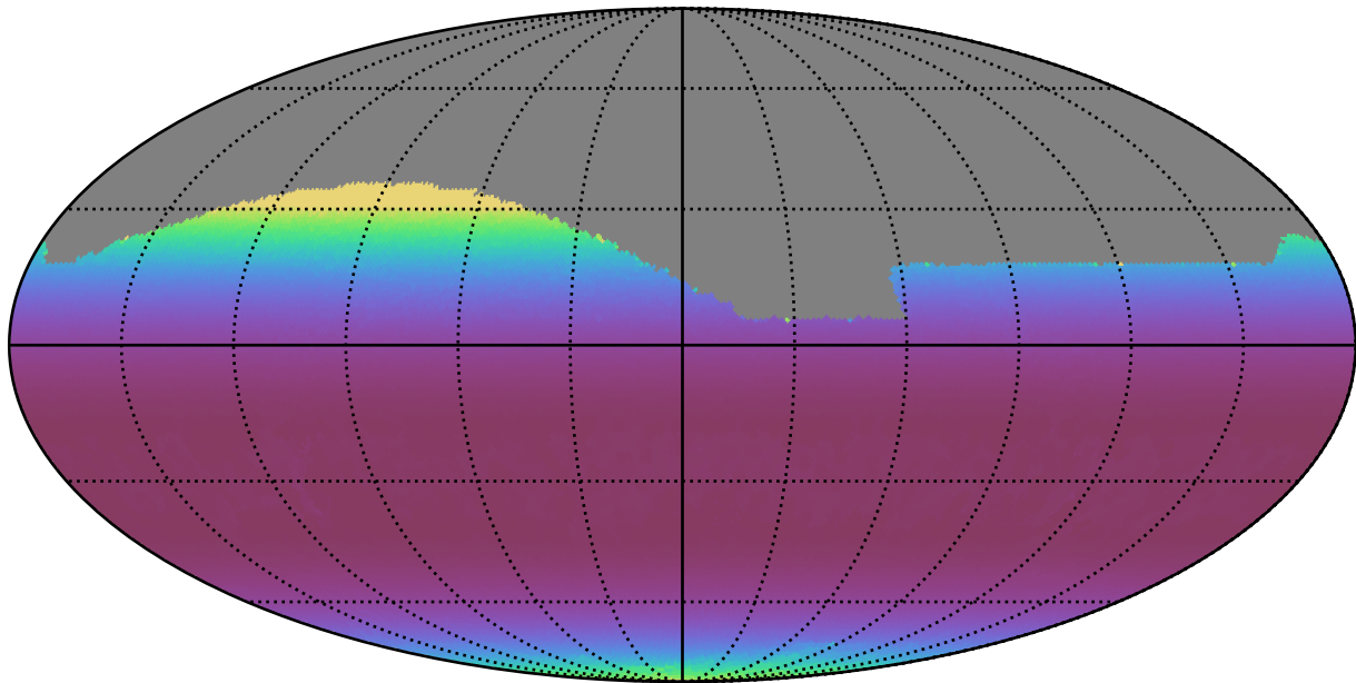
too_elab_r64_d2_gz_v3.4_10yrs All sky r band: Min airmass
